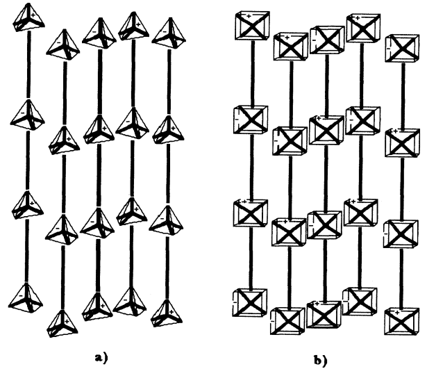
FIG. 2. Uniaxial chiral phases of a tetrahedral nematic LC: (a) C_3 helix, (b) C_2 helix.
