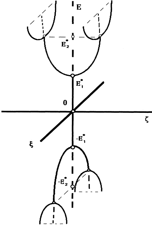
FIG. 5. Bifurcation tree of the Fréedericksz transition in tetrahedral nematic ( \mathbf{E} \parallel \bar{C}_4 ): \pm E_1^* and \pm E_2^* are the primary and the secondary bifurcation points, respectively.
