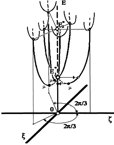
FIG. 6. Bifurcation tree of the Fréedericksz transition in tetrahedral nematic ( \mathbf{E} \parallel C_3 ): E_1^* and E_2^* are the primary and the secondary bifurcation points. A hysteresis is shown in the vicinity of E_1^* .
