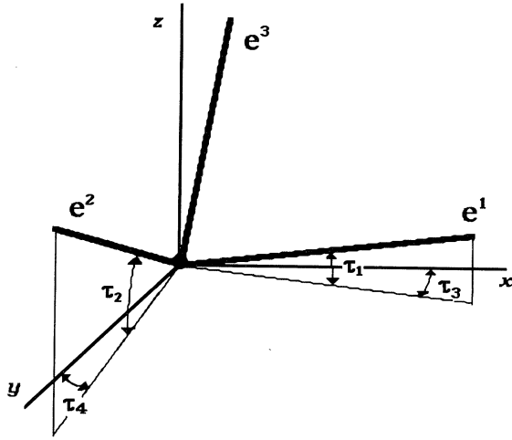
FIG. 4. A perturbed molecular "hedgehog."
