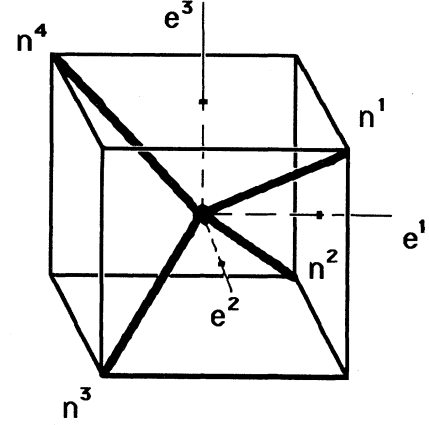
FIG. 1. Bonds in a tetrahedral nematic liquid crystal.
