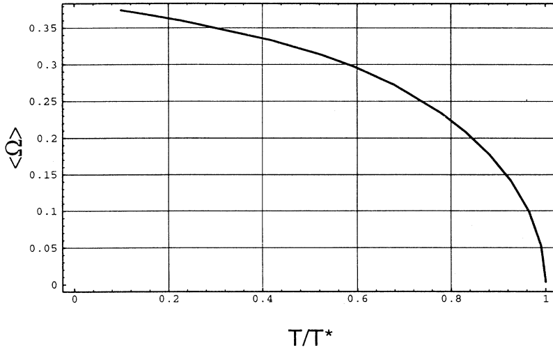
FIG. 3. Second order phase transition from isotropic liquid to the nonchiral tetrahedral nematic LC.
