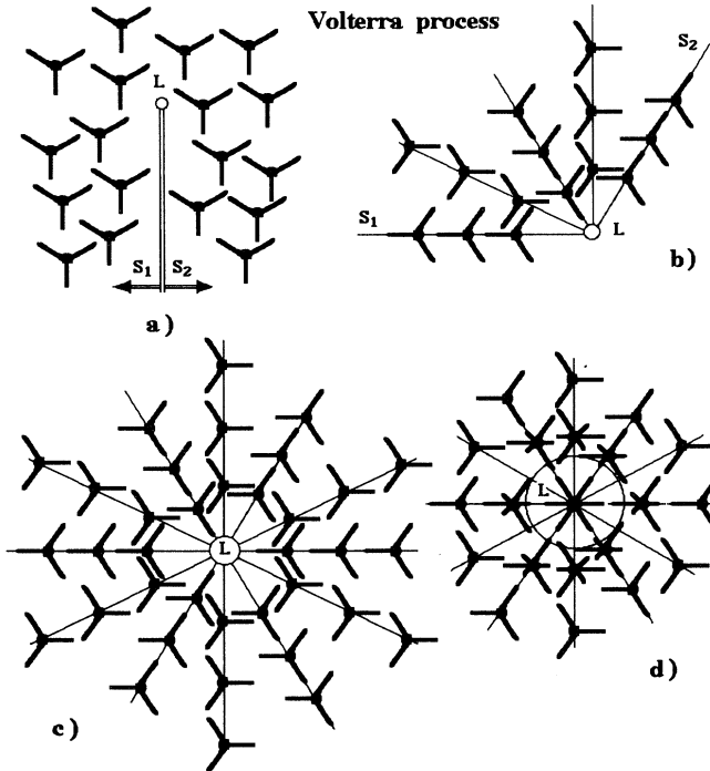
FIG. 7. The origin of the disclination line in the tetrahedral nematic via the Volterra process. Disclination line L is along the threefold rotational axis C_{3v} (normal to the plane of the page): (a) the cross section of the tetrahedral nematic LC by the plane L-S_1S_2 ; (b) the displacement of the lips L-S_1 and L-S_2 of the cutting surface with respect to each other; (c) the disclination line L after viscous relaxation of the structure; (d) disclination core.
